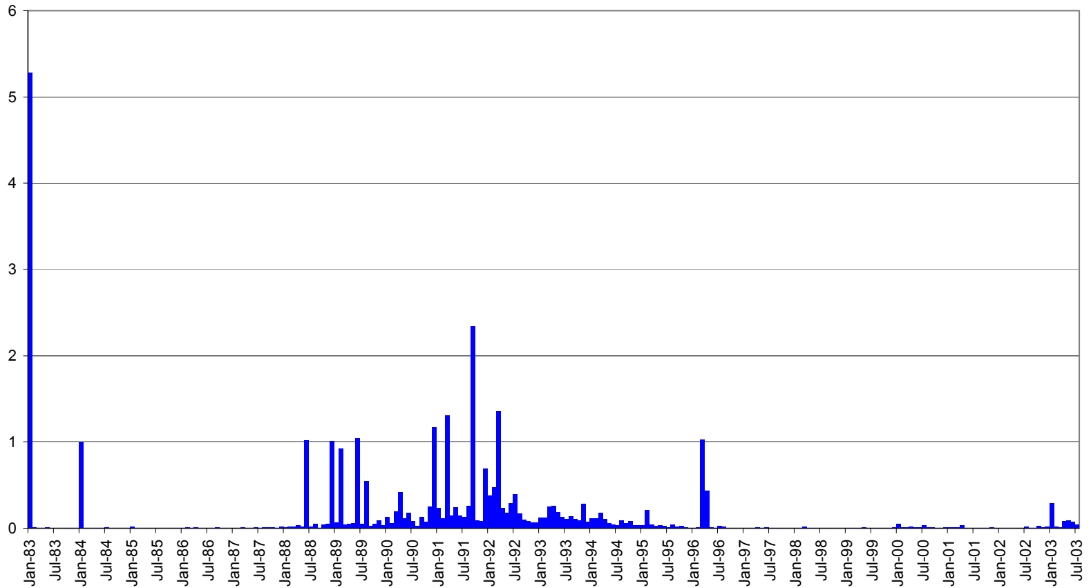
Age Distribution of Unadvertised Address Space (/8)
